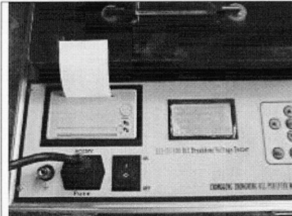
Photo 13. breakdown test finished and test result printed(Dirty oil)
